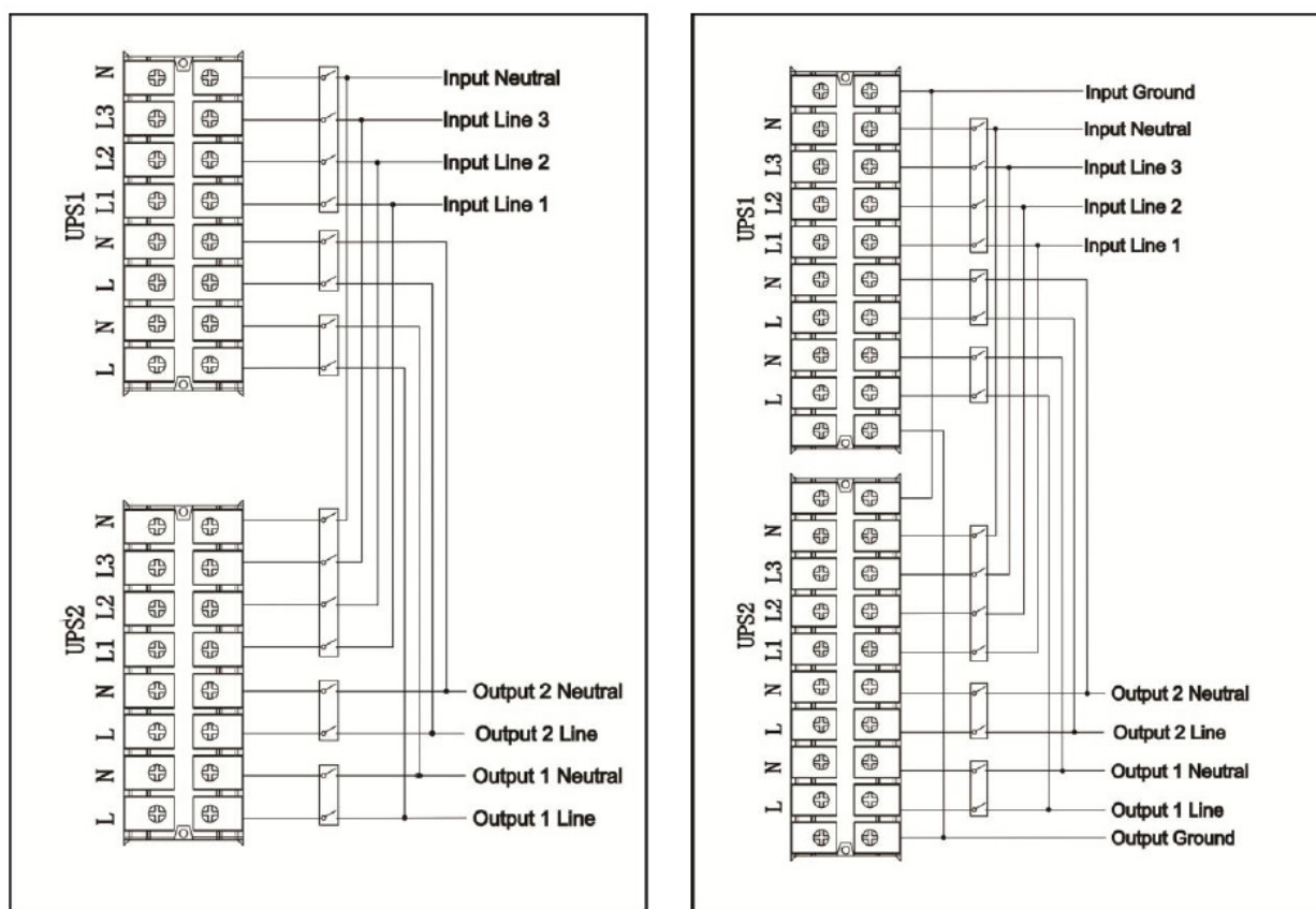
Figure 7 - Connections for Parallel System
