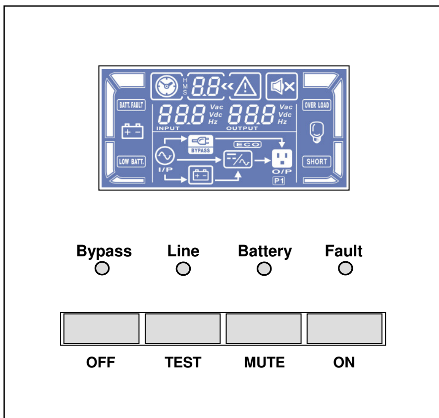
Figure 2 - Front panel
